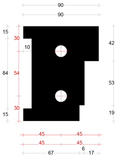
Neut links 90mm art. 2045469
