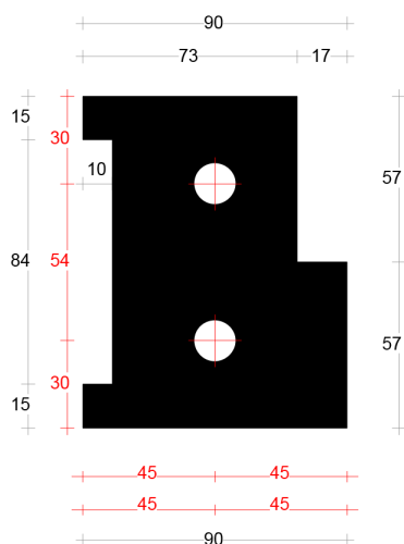
Neut links 90mm art. 2045434
