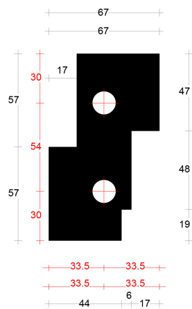
Tussenneut links 67mm art. 2045610
