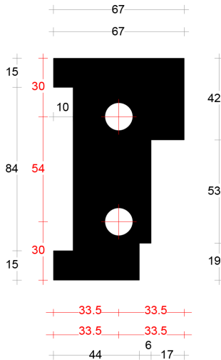
Neut links 67mm art. 2045466
