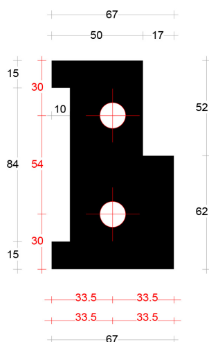
Neut links 67mm art. 2045375
