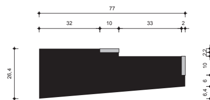
Vullat hefschuif 67.10 art. 2045485
