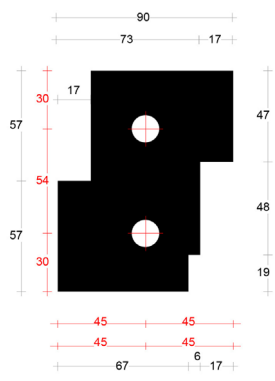
Tussenneut links 90mm art. 2045614
