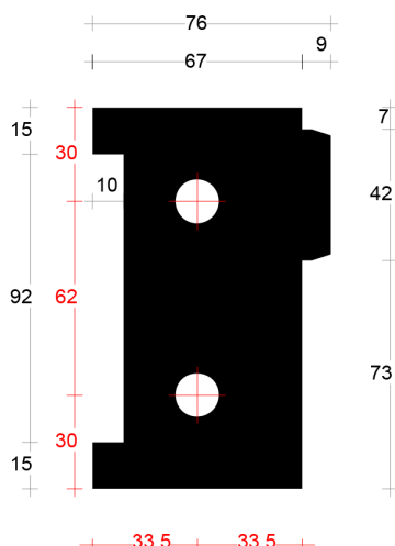
Neut schuifdeur links art. 2045455
