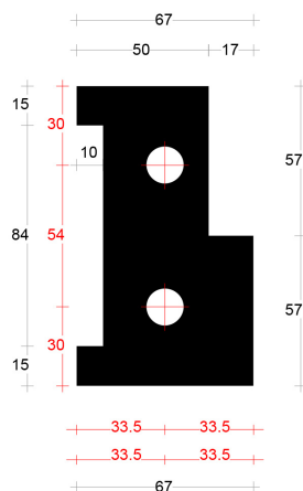
Eindneut links 67mm art. 2045612
